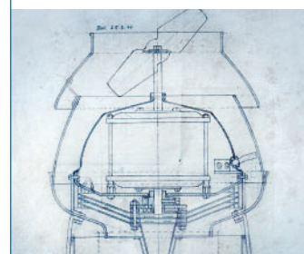
Defensor Rotary Disk Atomizer from 1948
